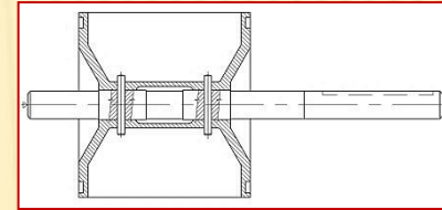
Rotor with side plates
